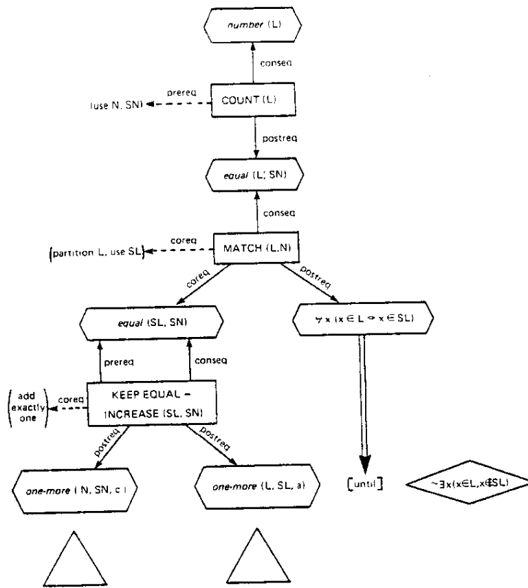
FIG. 4. Portion of planning net for standard counting.
