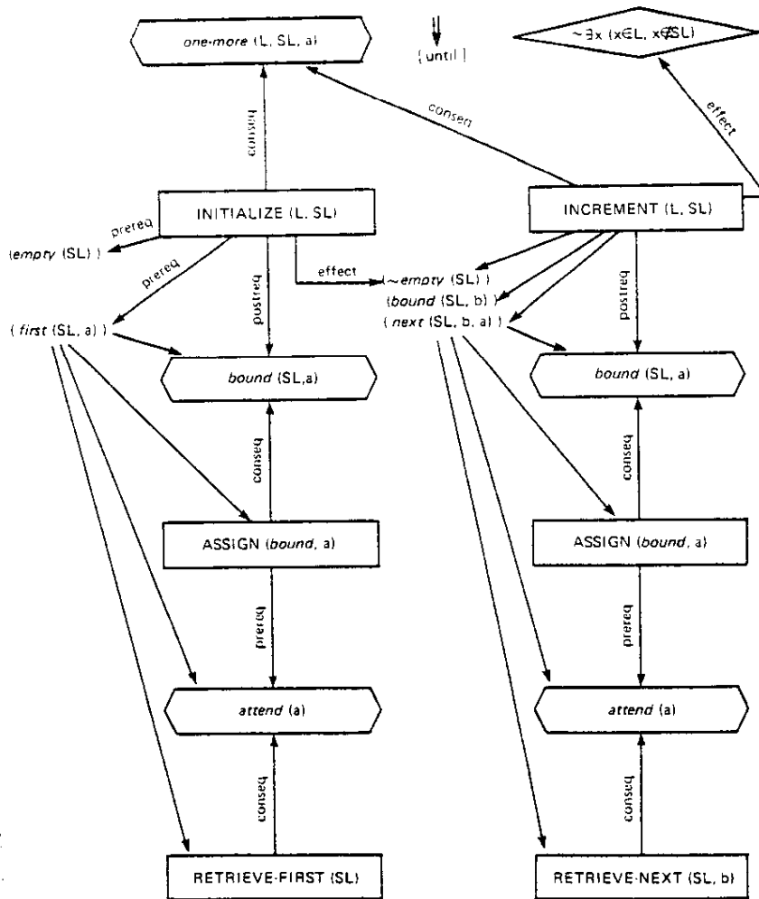
FIG. 5. Completion of planning for one-more ( L, SL, a ).
