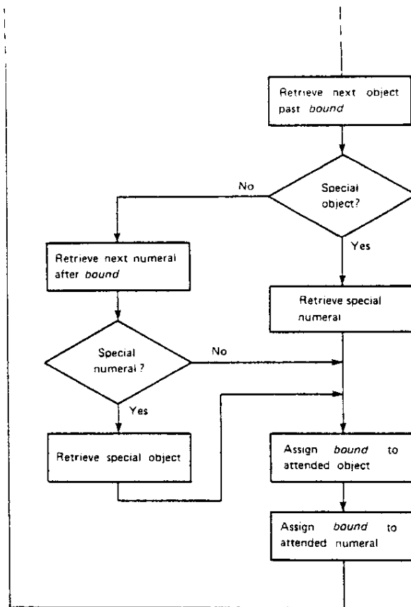
FIG. 6. Modified counting by Model SC-1.
