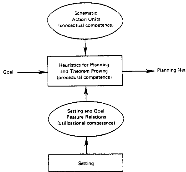
FIG. 1. Components of competence.
