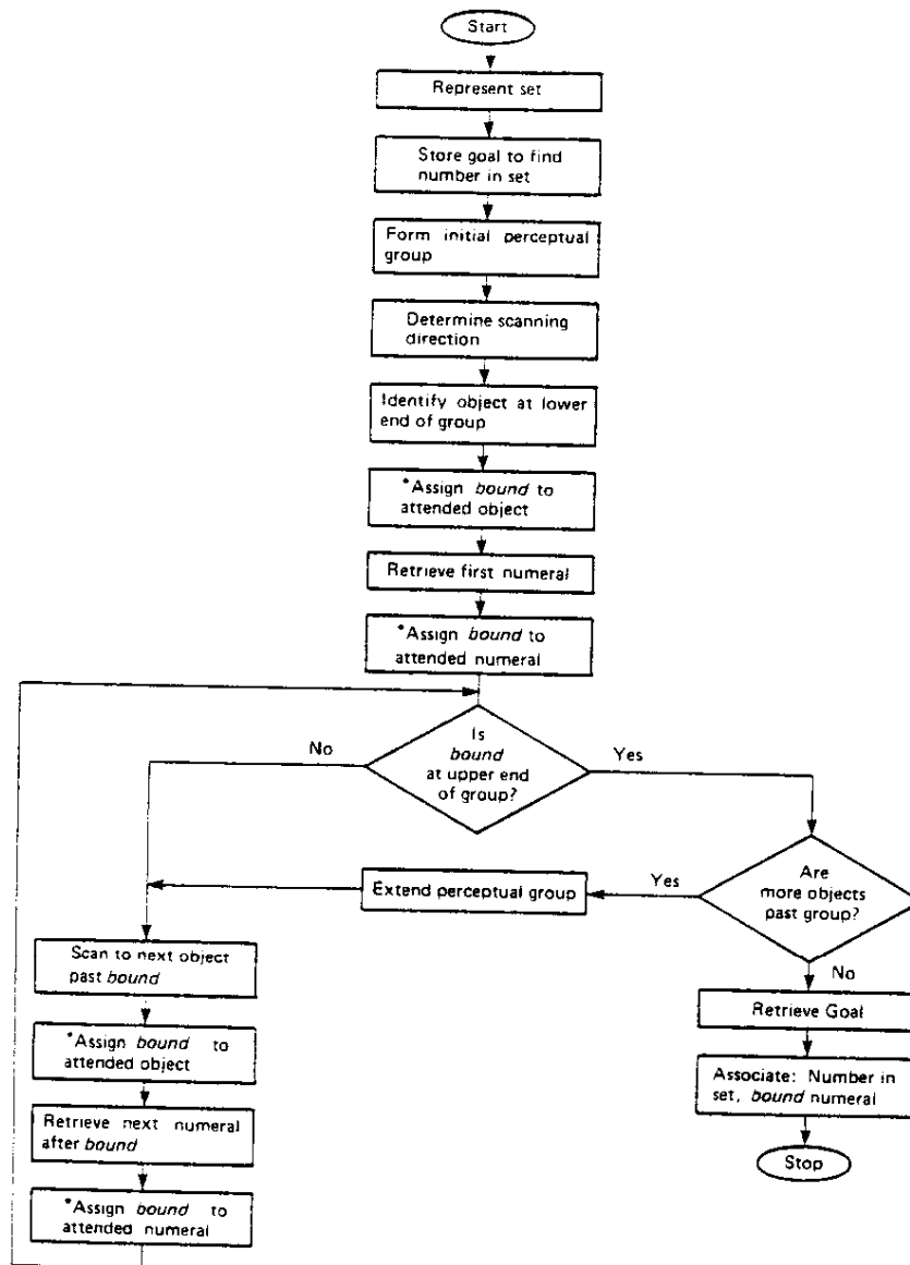
FIG. 9. Procedure for standard counting represented in SC. Prerequisites of components labeled with * may be violated by pairing constraint.
