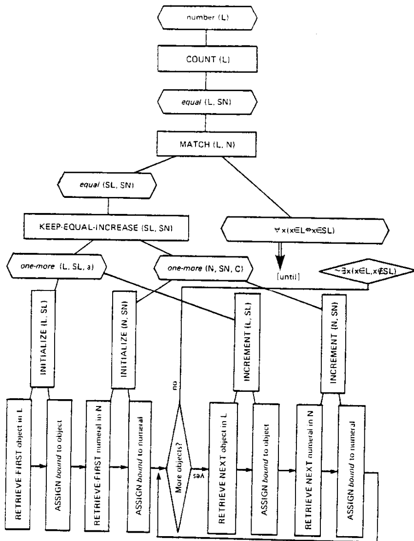
FIG. 3. Planning net for standard counting. SN denotes an initial segment of numerals; SL denotes an initial segment of objects.
