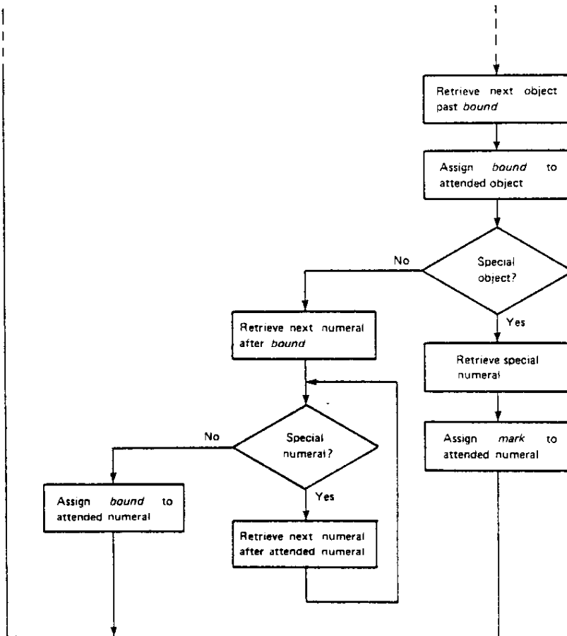
FIG. 7. Modified counting by Model SC-2.
