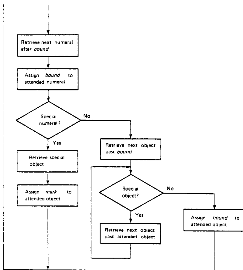
FIG. 8. Modified counting by Model SC-3.
