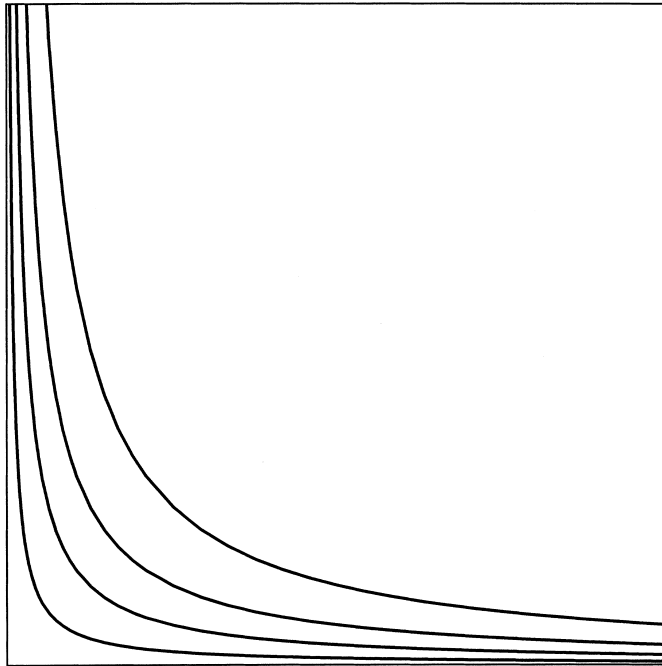
Fig. 5. Smoothing of a transversal intersection. A greater degree of smoothing leads to a lower magnitude of curvature at the curvature extremum.
